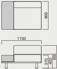
FN113-115L 1Pソファ+木製テーブル W1150 D800 H650 (SH400) mm rank1 ¥264,000 rank4 ¥276,000 rank2 ¥268,000 rank5 ¥280,000 rank3 ¥272,000
